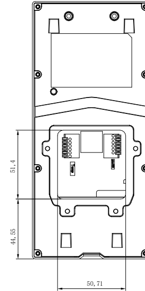
4 BACK VIEW
