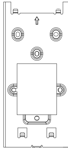
② FRONT VIEW:WALL MOUNTING BRACKET PLACEMENT
