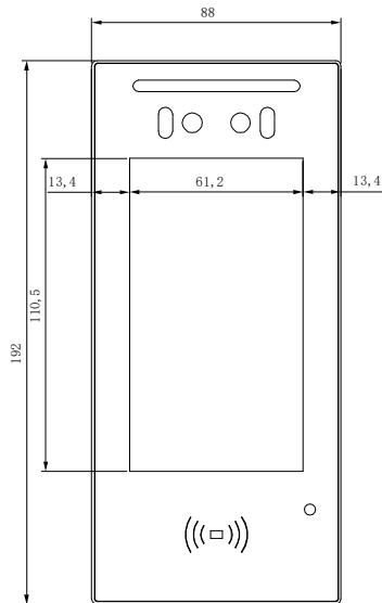
1 FRONT VIEW
