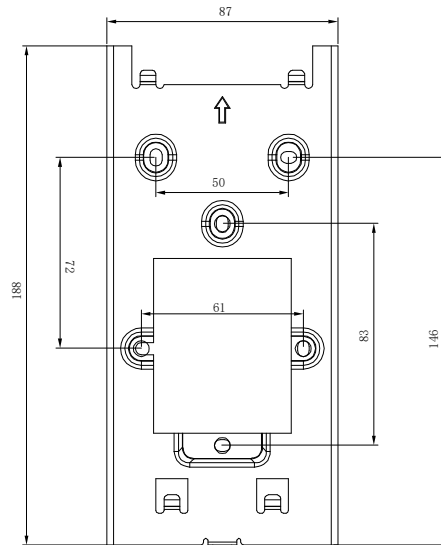
1 FRONT VIEW
